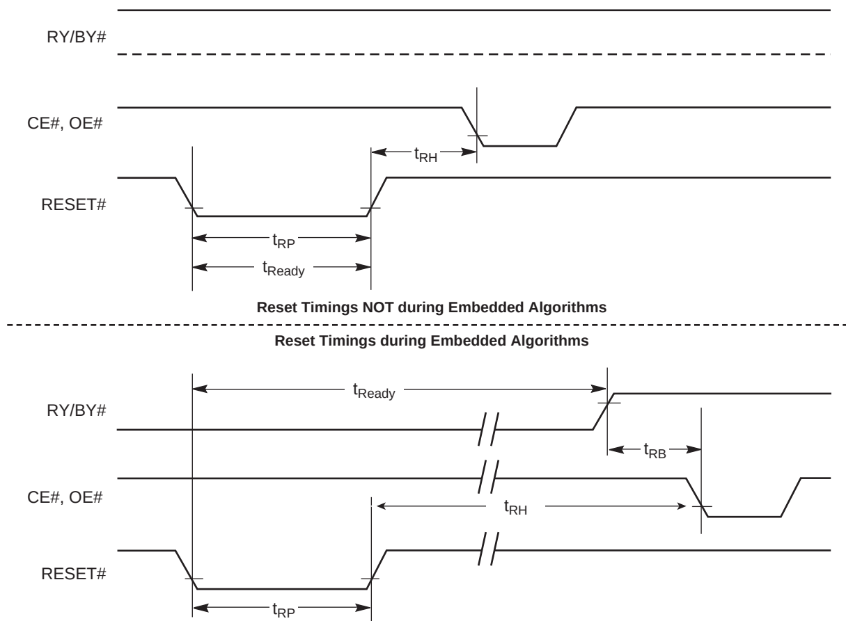
Figure 15.4 Reset Timings
