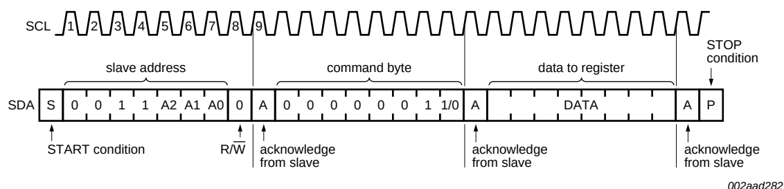
Fig 15. Write to I/O configuration or polarity inversion registers
