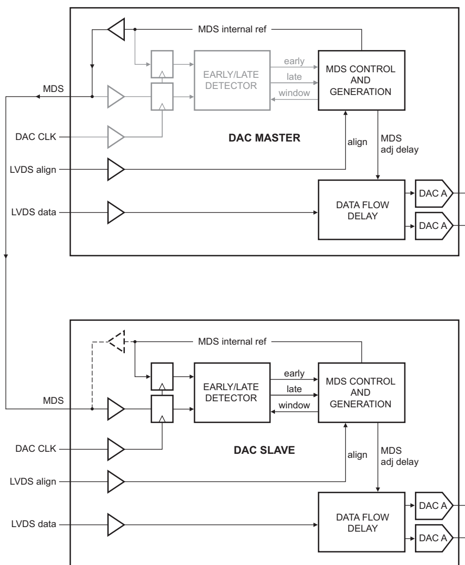
Fig 37. MDS synchronization
