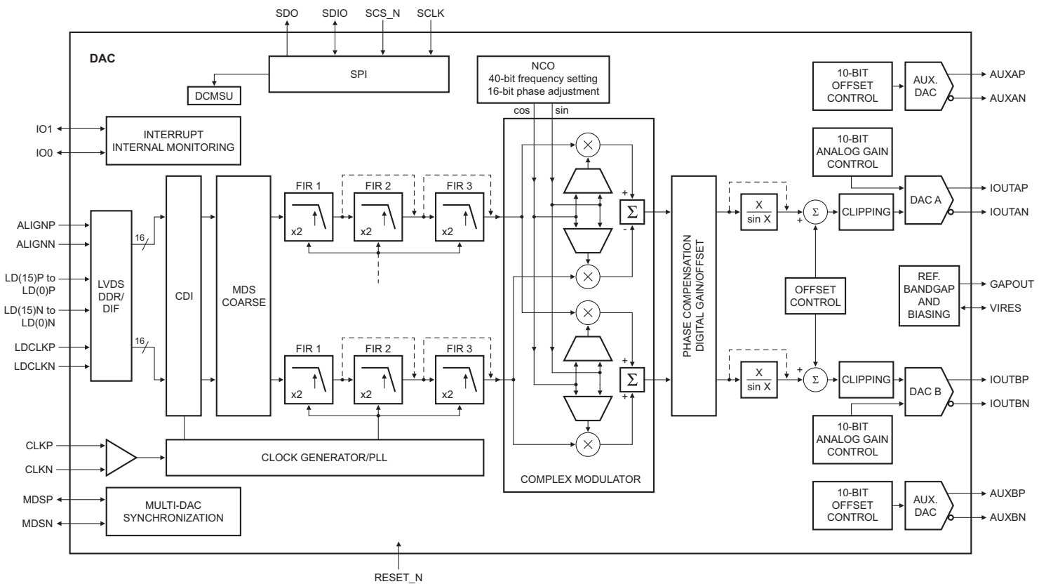
Fig 1. DAC1627D1G25 block diagram
