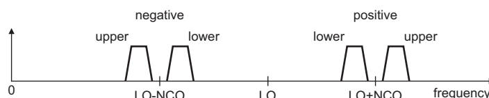
Fig 34. Complex modulation after LO mixing
