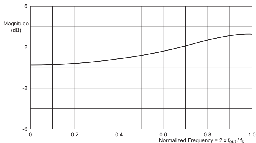
Fig 35. Inverse sin(x)/x response
