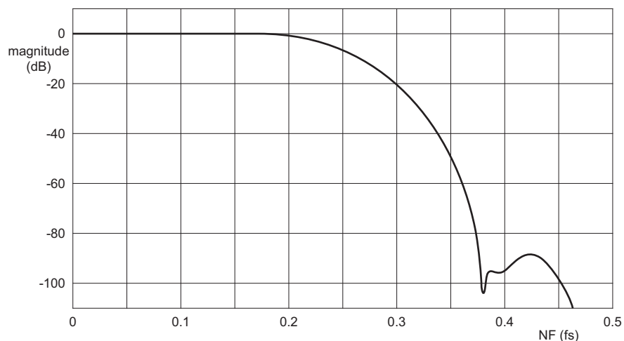
Fig 31. Second stage half-band filter response
