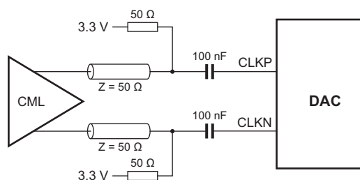
Fig 25. DAC core clock: CML configuration with AC-coupling
