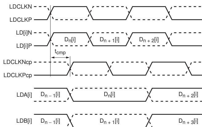
Fig 27. LVDS DDR demux timing (LVDS A and B paths not swapped; LDAB_SWAP = 0)
