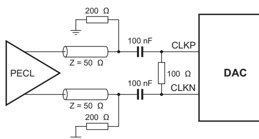
Fig 26. DAC core clock: PECL configuration with AC-coupling
