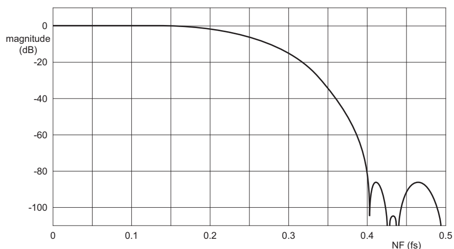
Fig 32. Third stage half-band filter response
