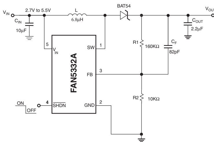
Figure 3. Test Circuit
