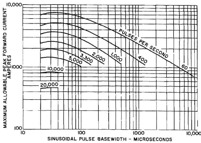
3. MAXIMUM ALLOWABLE FORWARD CURRENT SINUSOIDAL WAVEFORM ( T_C = 120^\circ\text{C} ) DOUBLE-SIDE COOLED
