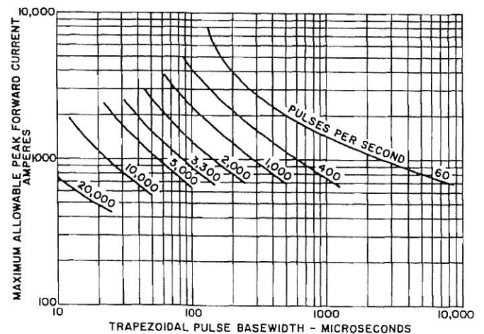
6. MAXIMUM ALLOWABLE PEAK FORWARD CURRENT TRAPEZOIDAL WAVEFORM ( T_C = 120^\circ\text{C} ) DI/DT (RISING & FALLING) = 100\text{ A}/\mu\text{s} DOUBLE-SIDE COOLED
