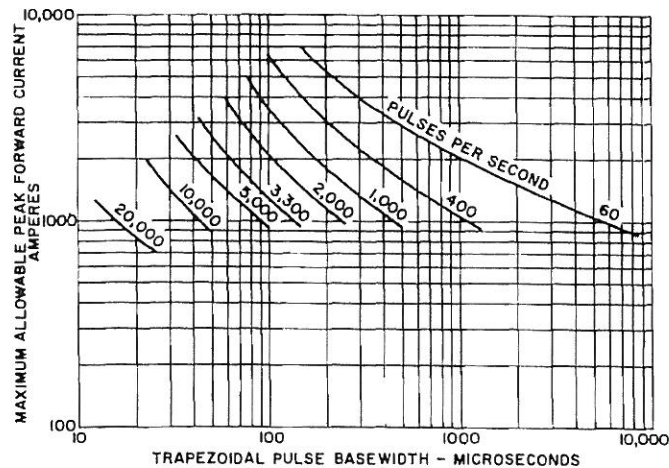
5. MAXIMUM ALLOWABLE PEAK FORWARD CURRENT TRAPEZOIDAL WAVEFORM ( T_C = 95^\circ\text{C} ) DI/DT (RISING & FALLING) = 100\text{ A}/\mu\text{s} DOUBLE-SIDE COOLED
