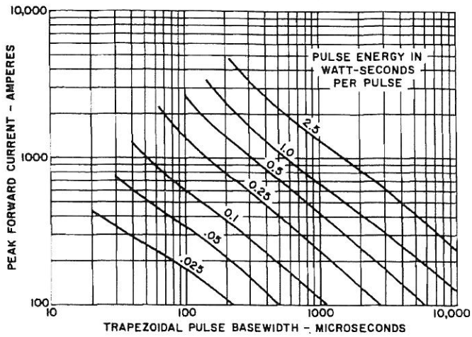
7. TRAPEZOIDAL PULSE ENERGY DI/DT (RISING & FALLING) = 100 \text{ A}/\mu\text{s} ( T_J = 175^\circ\text{C} )
