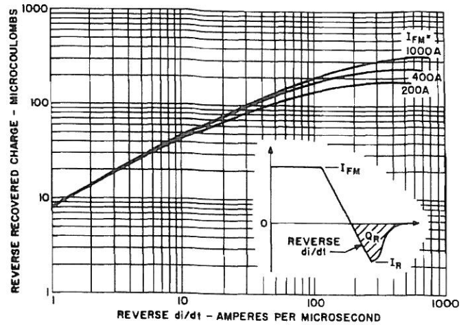
8. TYPICAL RECOVERED CHARGE ( T_J = 175^\circ\text{C} ) FOR PARTS SUPPLIED VIA A398-X9 PART NUMBER, GRAPH 8 REPRESENTS A MAXIMUM RECOVERED CHARGE ( T_J = +175^\circ\text{C} )
