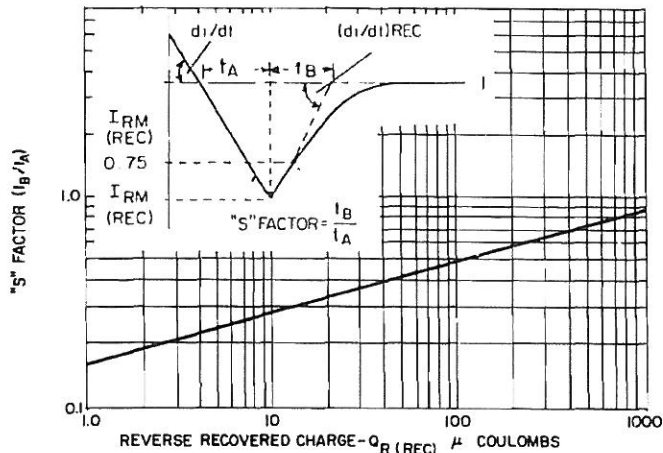
9. TYPICAL "S" FACTOR VERSUS RECOVERY CHARGE ( T_J = 175^\circ\text{C} )
