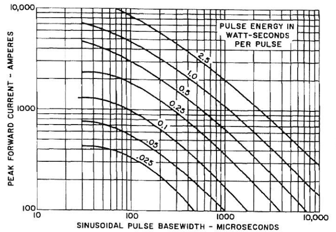
4. SINUSOIDAL PULSE ENERGY ( T_J = 175^\circ\text{C} )
