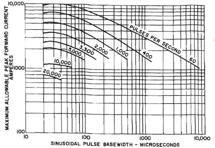
2. MAXIMUM ALLOWABLE PEAK FORWARD CURRENT SINUSOIDAL WAVEFORM ( T_C = 95^\circ\text{C} ) DOUBLE-SIDE COOLED
