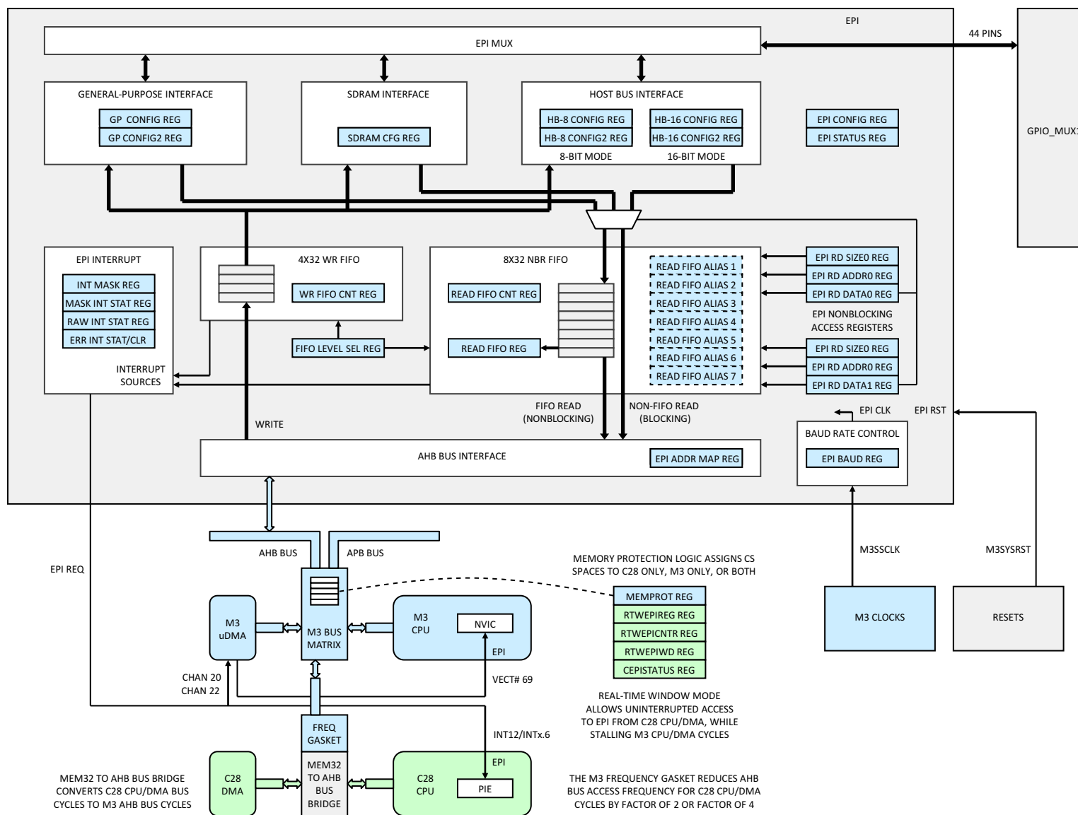
Figure 5-16. EPI
