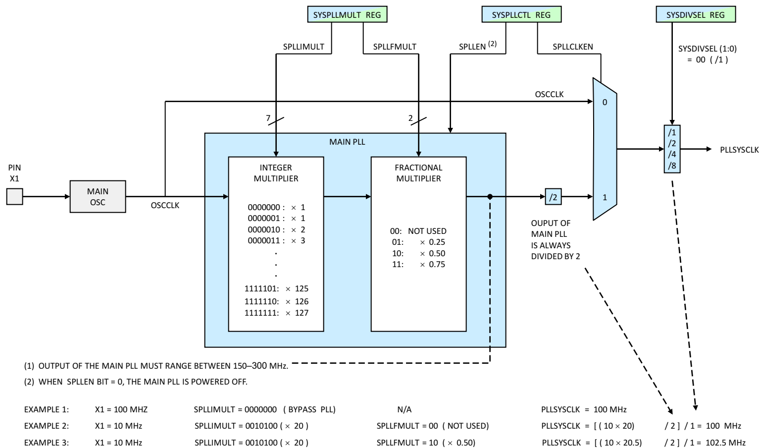
Figure 6-8. Main PLL
