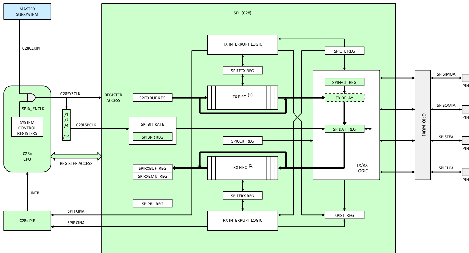
Figure 5-50. SPI (C28x)
