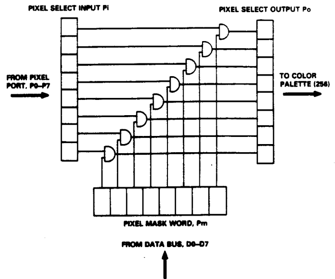
Figure 4. Internal Architecture of Pixel Input Port
