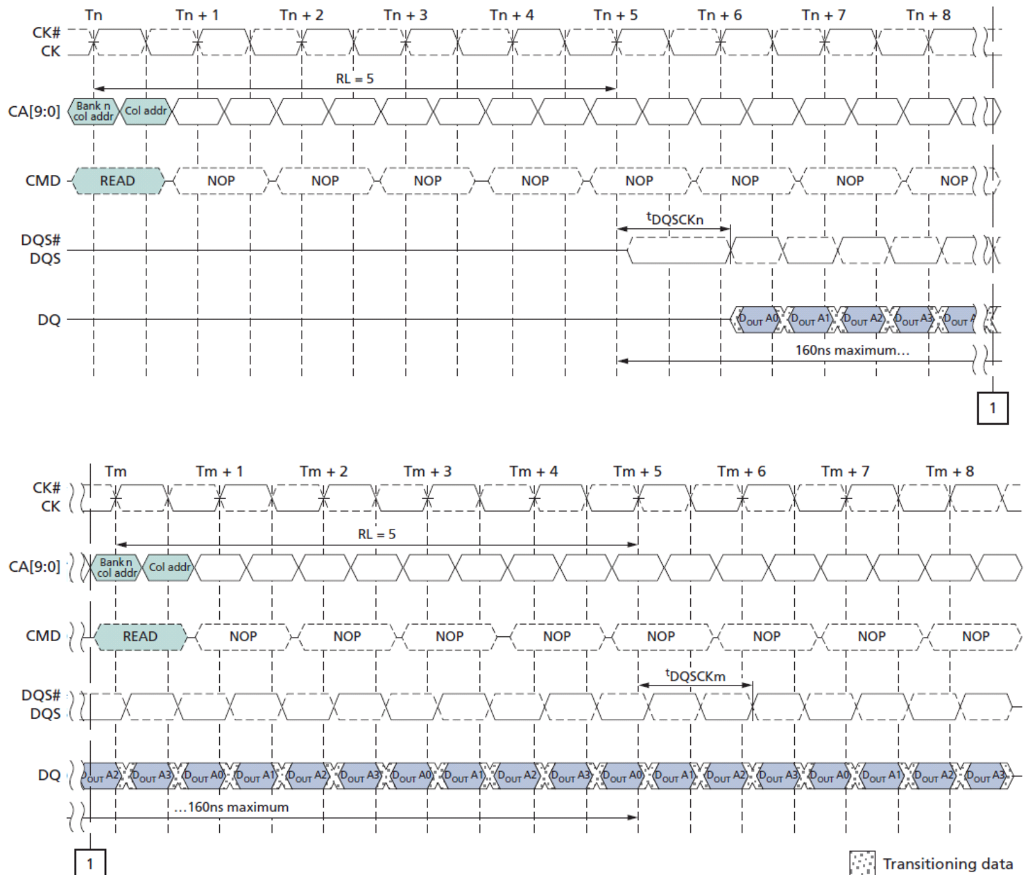
Figure 10 : tDQSKDS Timing
