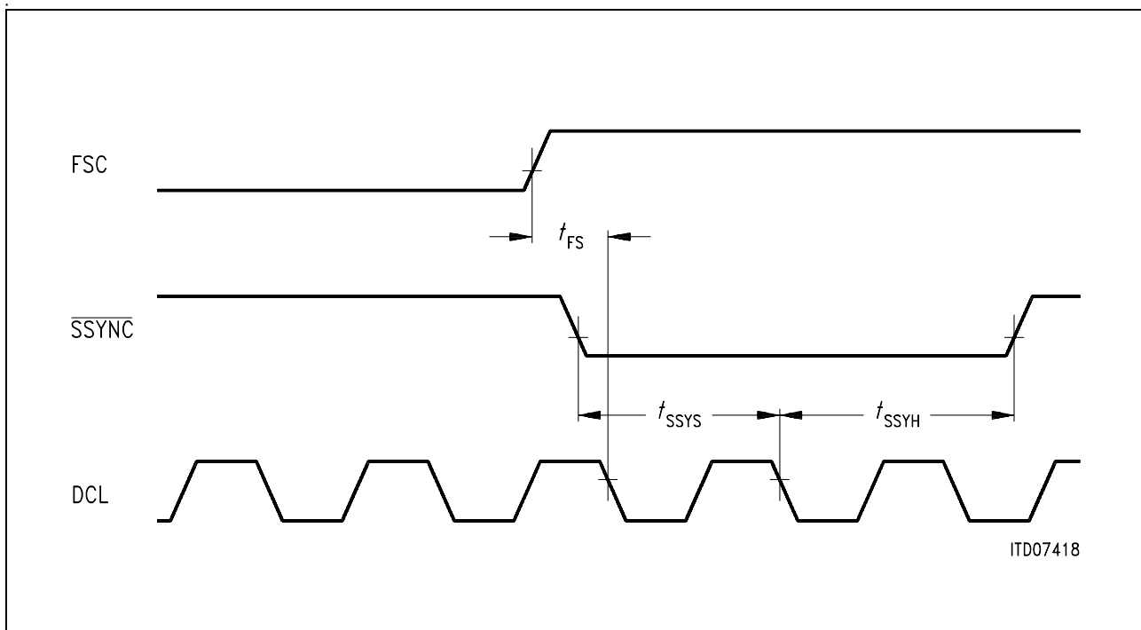
Figure 5-8 SSYNC Timing
