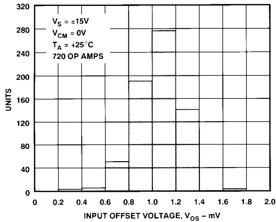
Figure 2. OP292 Input Offset Voltage Distribution @ \pm 15 V
