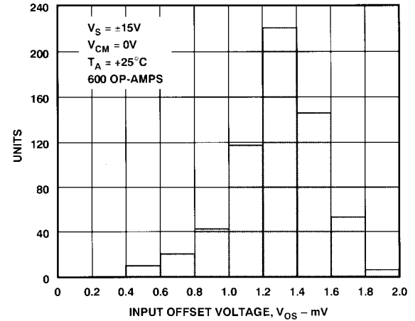
Figure 5. OP492 Input Offset Voltage Distribution @ \pm 15 V
