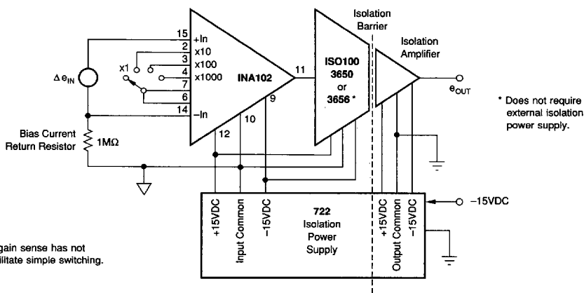
FIGURE 10. Precision Isolated Instrumentation Amplifier.
