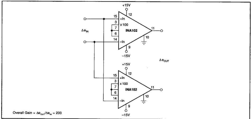
FIGURE 15. Differential Input/Differential Output Amplifier (twice the gain of one INA).
