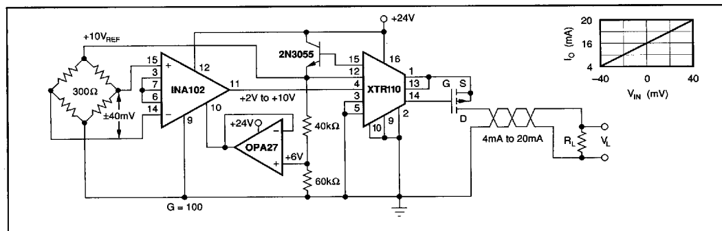
FIGURE 12. 4mA to 20mA Bridge Transmitter Using Single Supply Instrumentation Amplifier.
