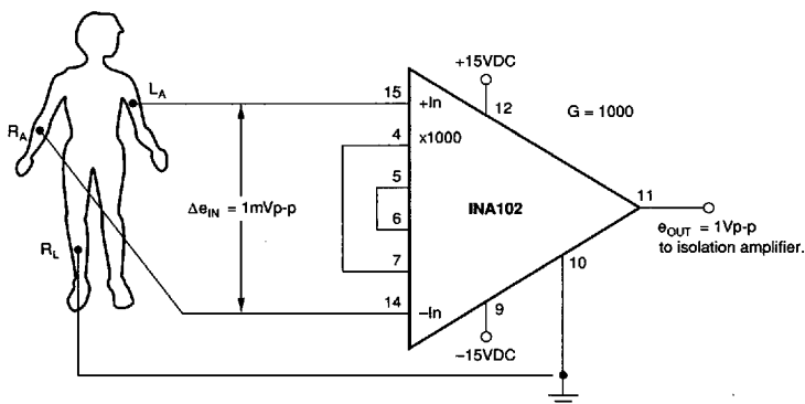
FIGURE 8. ECG Amplifier or Recorder Preamp for Biological Signals.
