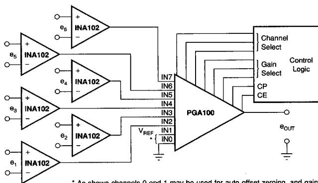
FIGURE 11. Multiple Channel Precision Instrumentation Amplifier with Programmable Gain.
