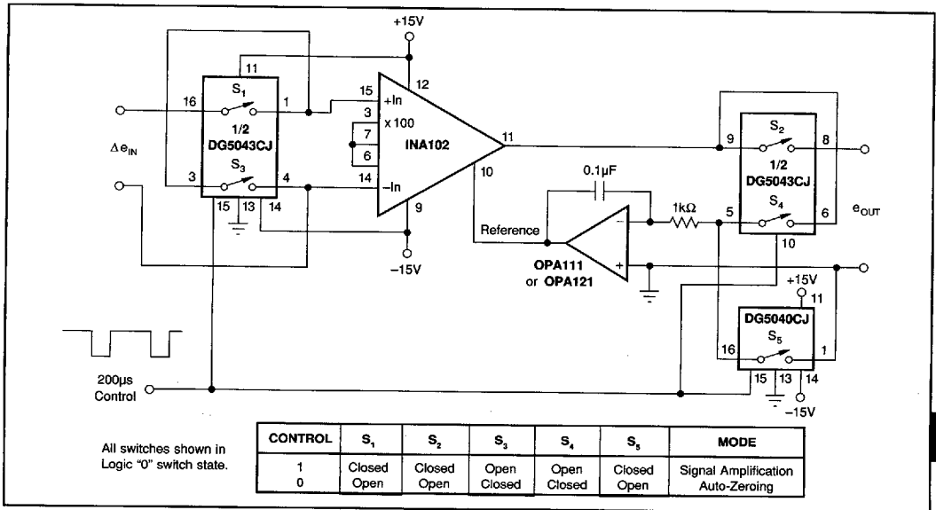
FIGURE 16. Auto-Zeroing Instrumentation Amplifier Circuit.
