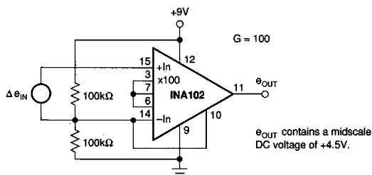
FIGURE 9. Single Supply Low Power Instrumentation Amplifier.
