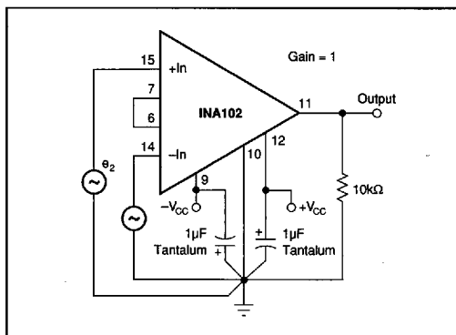
FIGURE 2. Basic Circuit Connection for the INA102.
