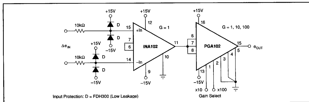
FIGURE 13. Programmable-Gain Instrumentation Amplifier Using the INA102 and PGA102.
