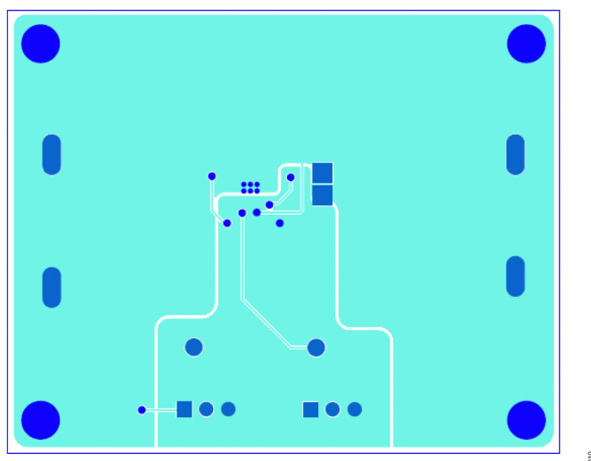
Figure 10. Bottom Layer, Recommended Layout
