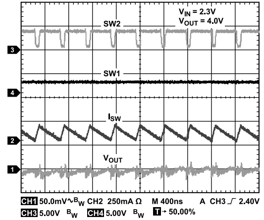
Figure 5. Boost Operation, V_{IN} = 2.3\text{ V} , V_{OUT} = 4.0\text{ V} , PWM
