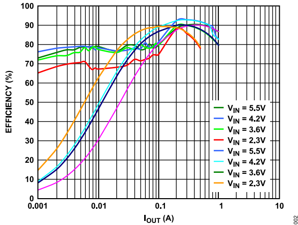
Figure 2. Efficiency vs. Load, V_{OUT} = 3.3\text{ V} , PWM and PSM
