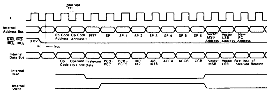
Figure 10 Interrupt Sequence
