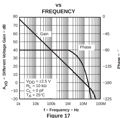
DIFFERENTIAL VOLTAGE GAIN AND PHASE
