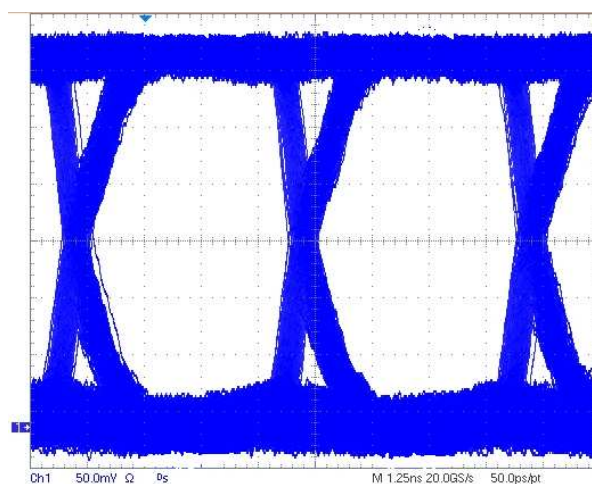
Figure 13. SN65LVDS348 Eye Pattern Running at 200 Mxfr/s
