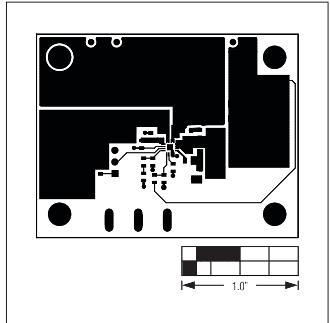
Figure 3. MAX15041 EV Kit PCB Layout—Component Side
