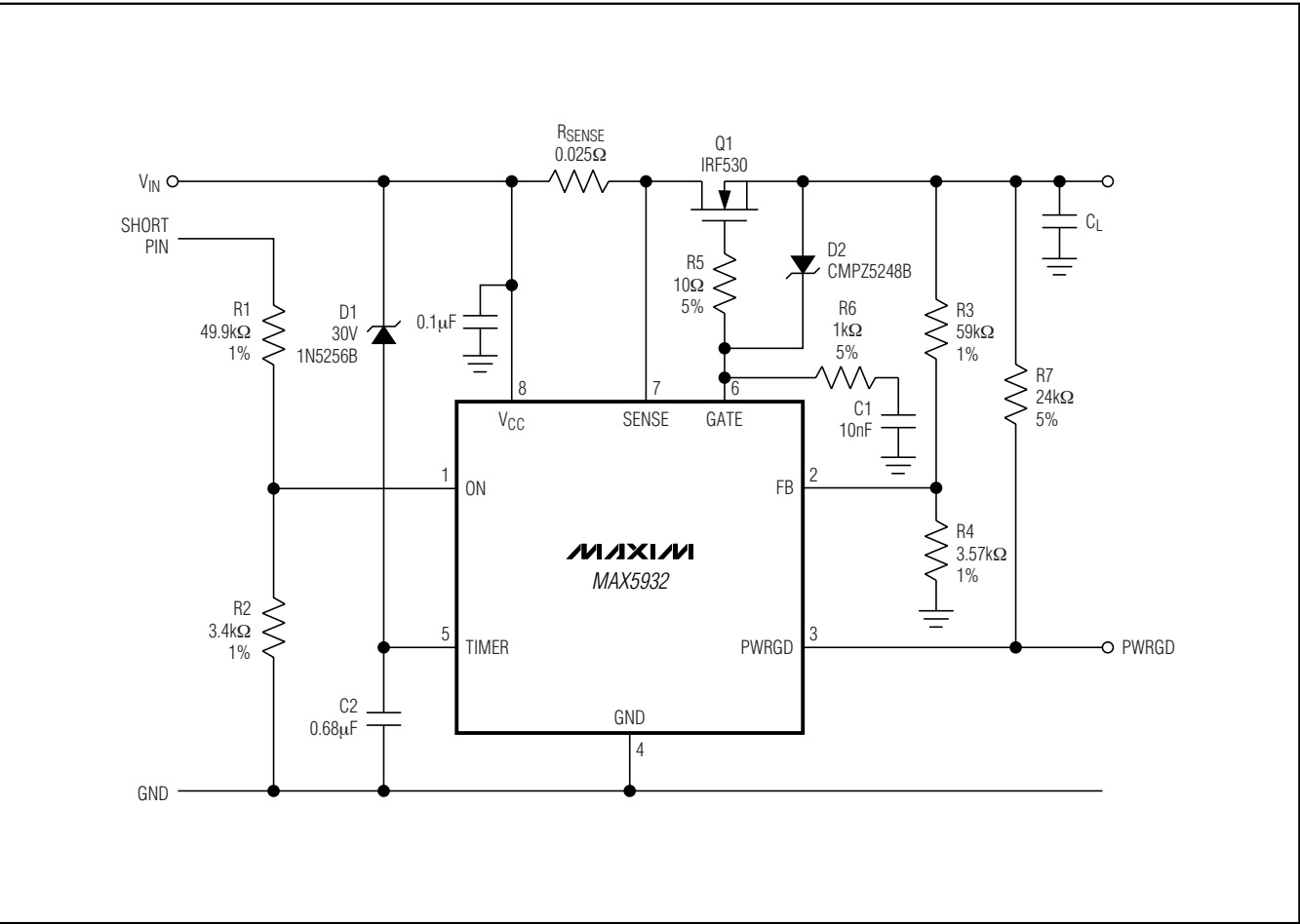
Figure 10. Overvoltage Detection
