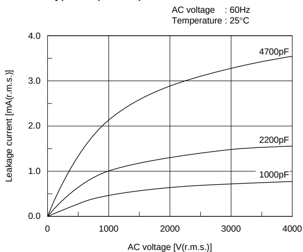
Type KJ (E char.)
