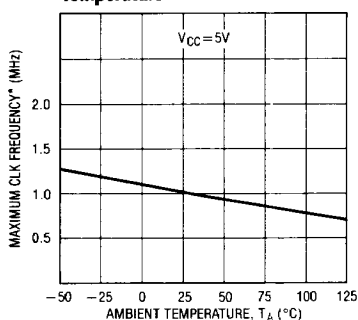
Maximum Clock Rate vs Temperature
