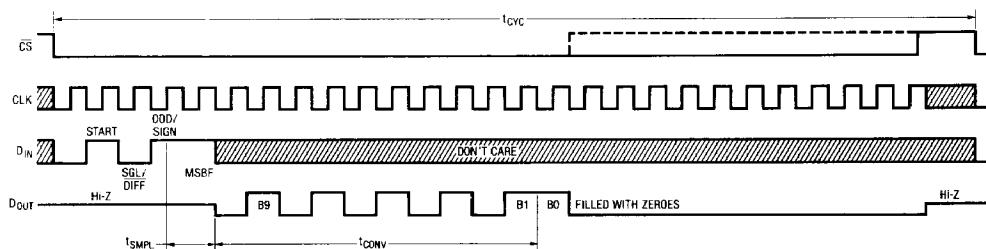
LTC1091 Operating Sequence Example: Differential Inputs (CH1 +, CH0 -)
