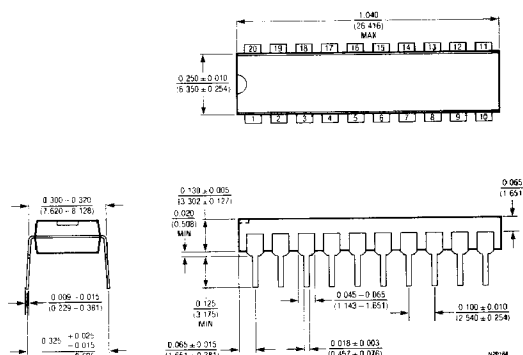
N Package 20 Lead Plastic DIP
