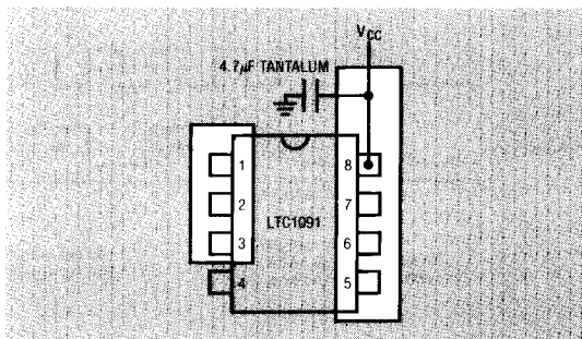
Figure 4. Example Ground Plane for the LTC1091
