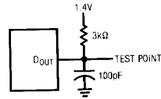
Load Circuit for t_{dDO} , t_r , and t_f
