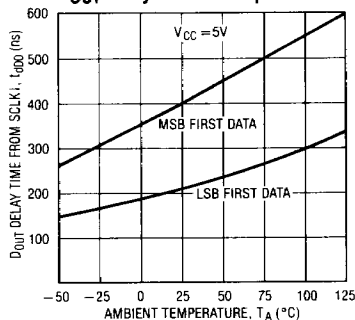
DOUT Delay Time vs Temperature
