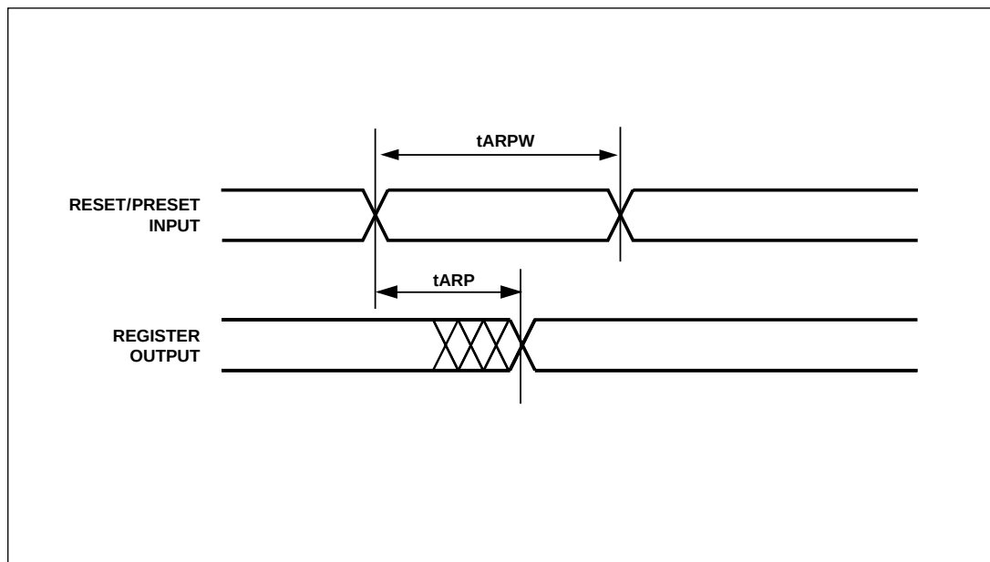
Figure 47. Asynchronous Reset/Preset
