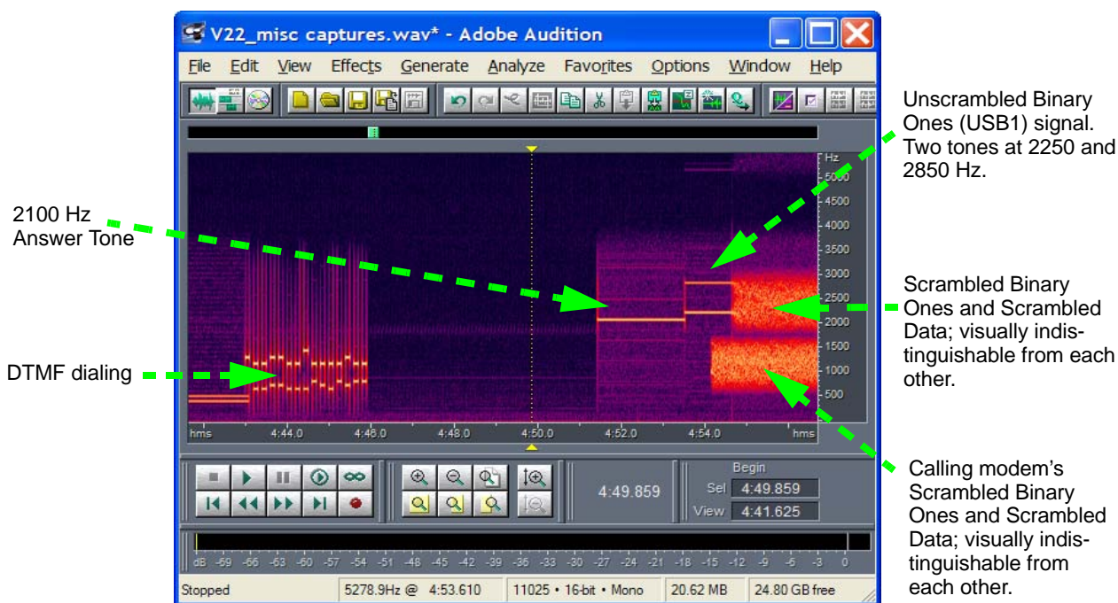
Figure 62. Appearance of V.22 Protocol
