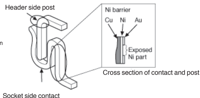
Socket side contact
