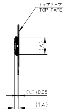
SECTION Y-Y
