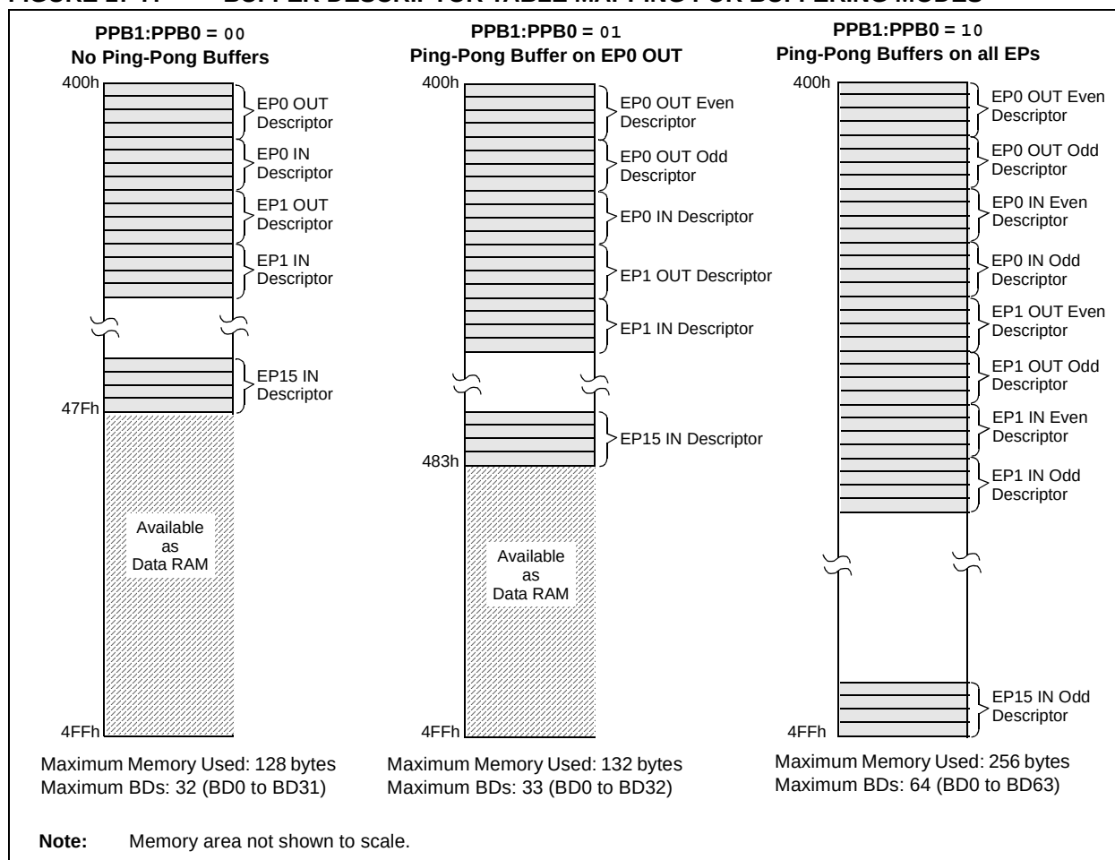
FIGURE 17-7: BUFFER DESCRIPTOR TABLE MAPPING FOR BUFFERING MODES
