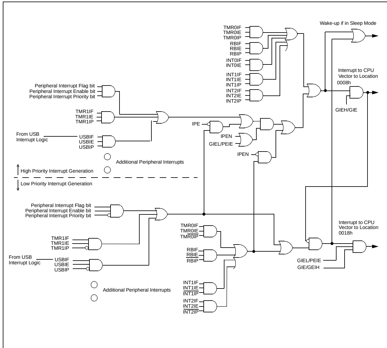
FIGURE 9-1: INTERRUPT LOGIC
