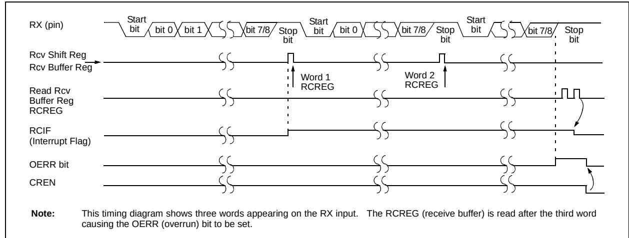
FIGURE 20-7: ASYNCHRONOUS RECEPTION
