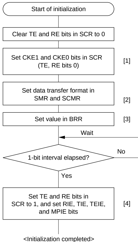
Figure 15.5 Sample SCI Initialization Flowchart
