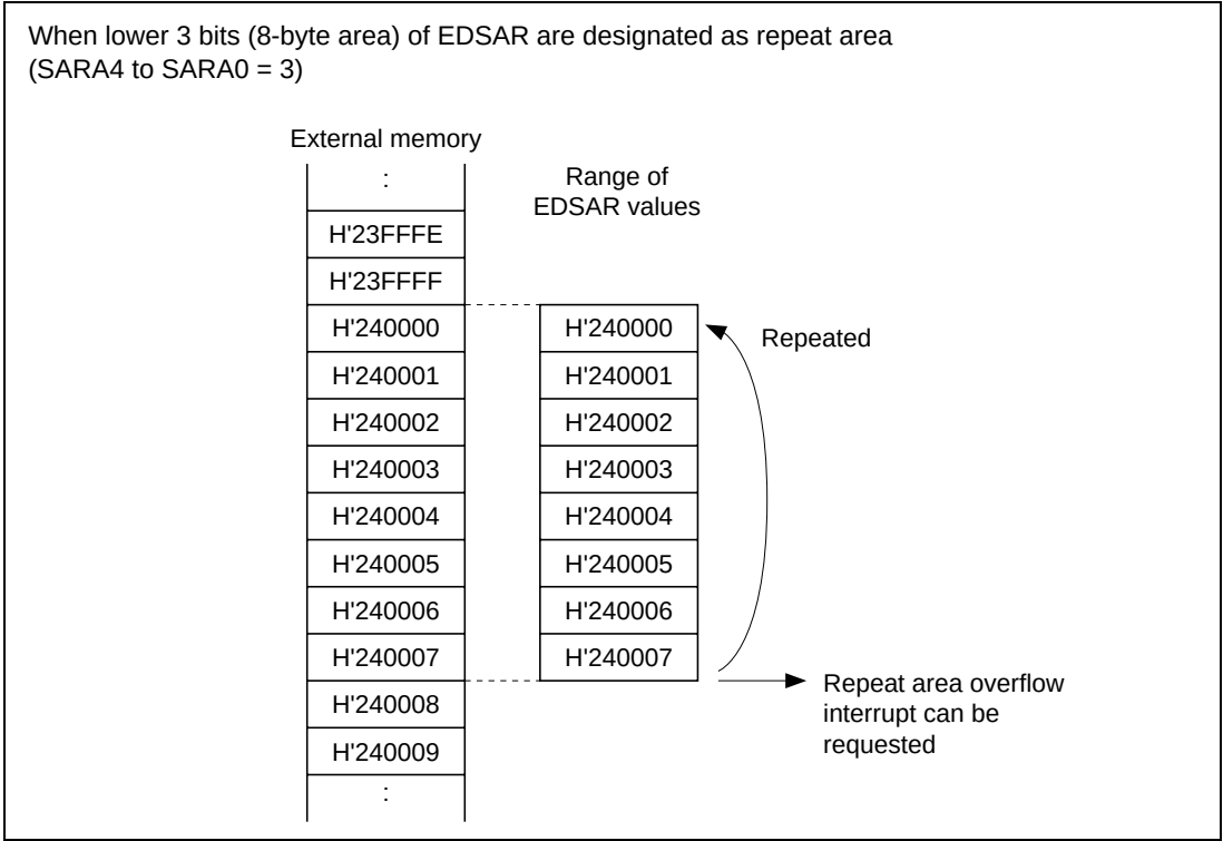
Figure 8.9 Example of Repeat Area Function Operation
