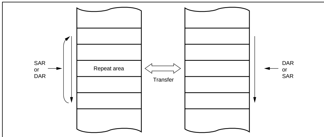
Figure 9.6 Memory Mapping in Repeat Mode
