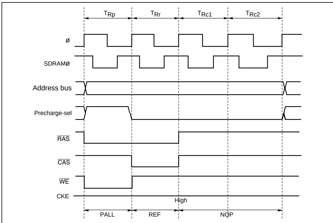
Figure 6.54 Auto Refresh Timing
