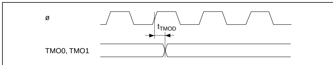
Figure 24.38 8-Bit Timer Output Timing
