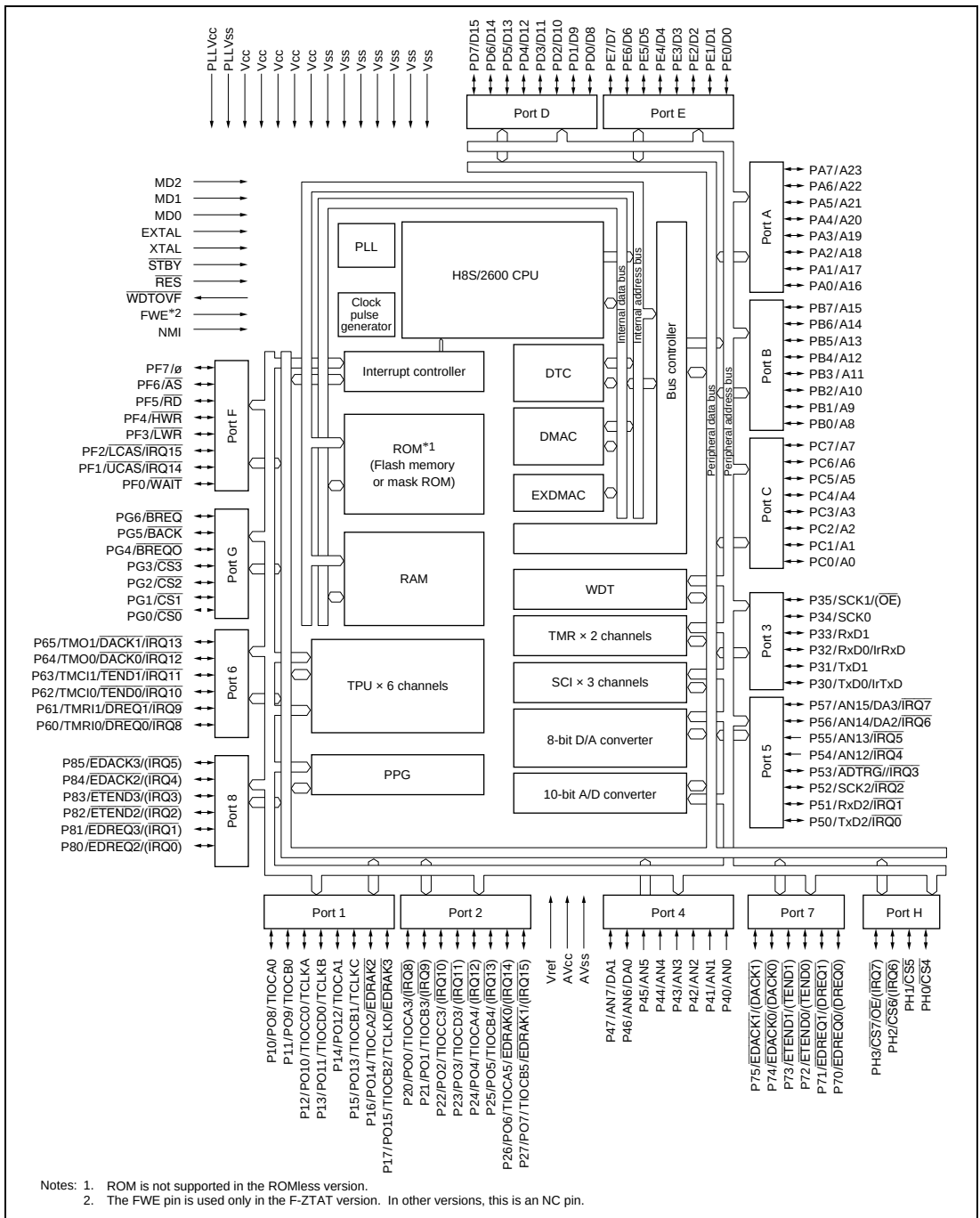
Figure 1.1 H8S/2678 Series Internal Block Diagram
