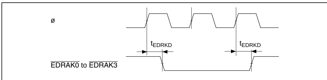
Figure 24.33 EXDMAC \overline{EDRAK} Output Timing
