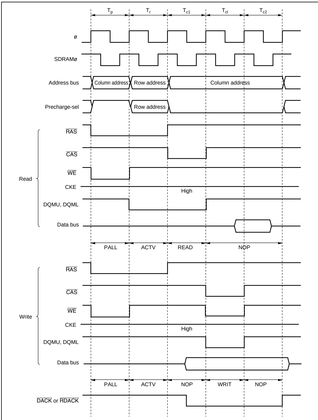
Figure 6.60 Example of \overline{\text{DACK}}/\overline{\text{EDACK}} Output Timing when DDS = 1 or EDDS = 1
