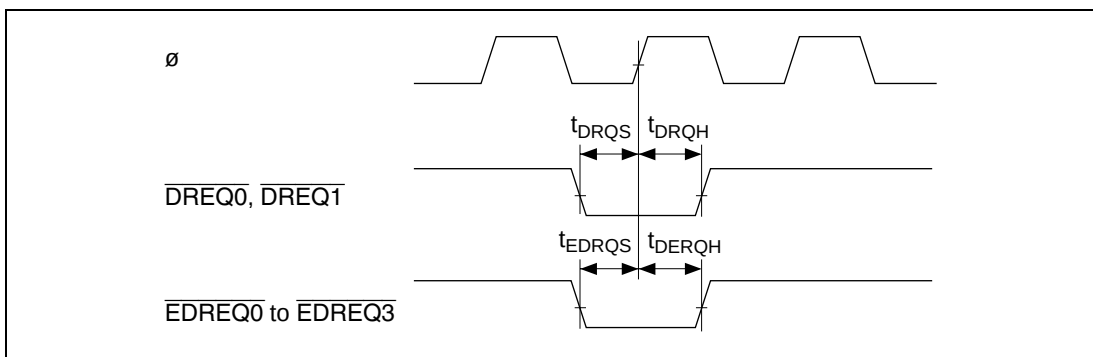
Figure 24.32 DMAC and EXDMAC \overline{DREQ} / \overline{EDREQ} Input Timing
