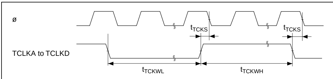
Figure 24.37 TPU Clock Input Timing
