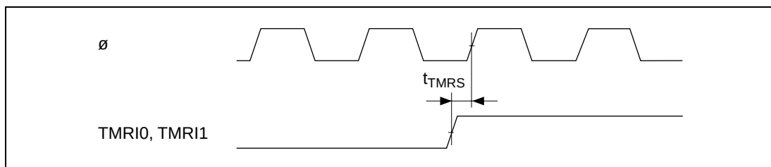
Figure 24.40 8-Bit Timer Reset Input Timing
