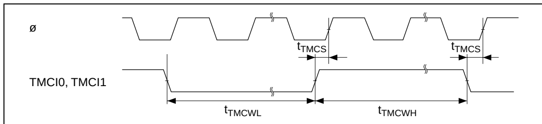
Figure 24.39 8-Bit Timer Clock Input Timing
