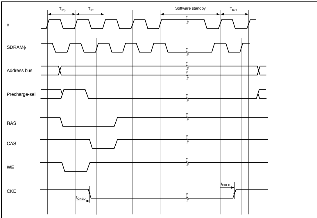
Figure 24.27 Synchronous DRAM Self-Refresh Timing
