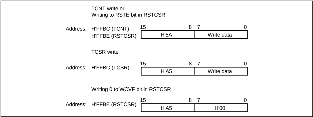
Figure 14.4 Writing to TCNT, TCSR, and RSTCSR
