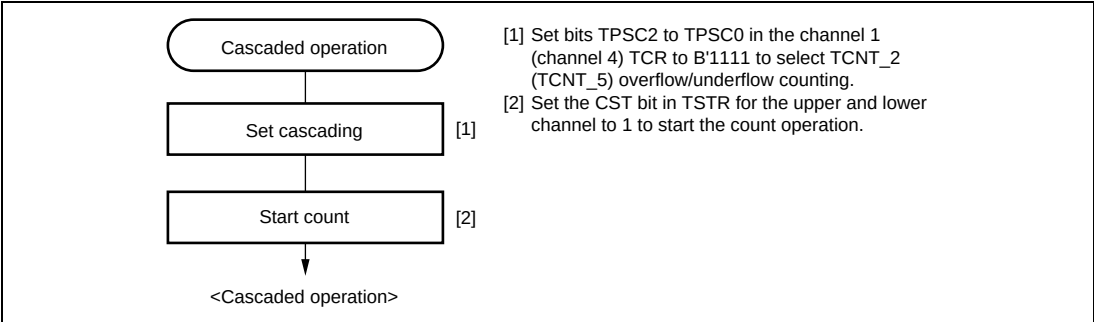
Figure 11.17 Cascaded Operation Setting Procedure
