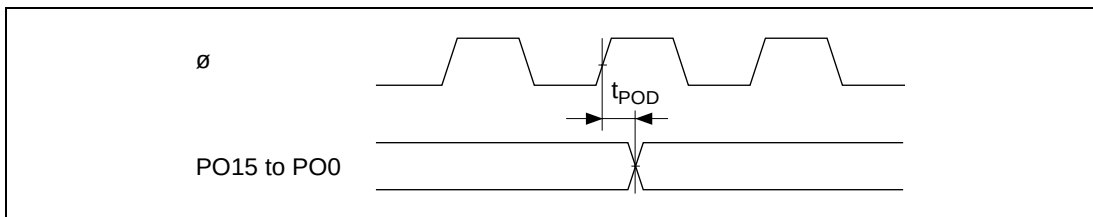
Figure 24.35 PPG Output Timing
