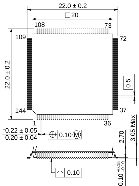
Figure C.2 Package Dimensions (FP-144G)
