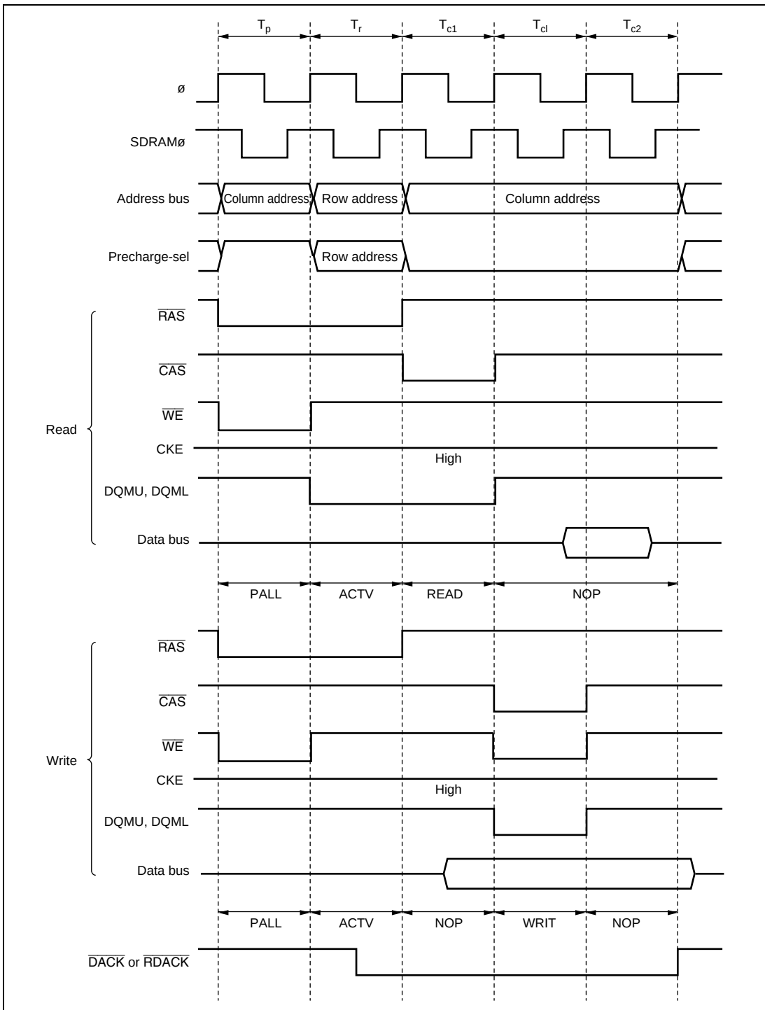
Figure 6.61 Example of \overline{\text{DACK}}/\overline{\text{EDACK}} Output Timing when DDS = 0 or EDDS = 0
