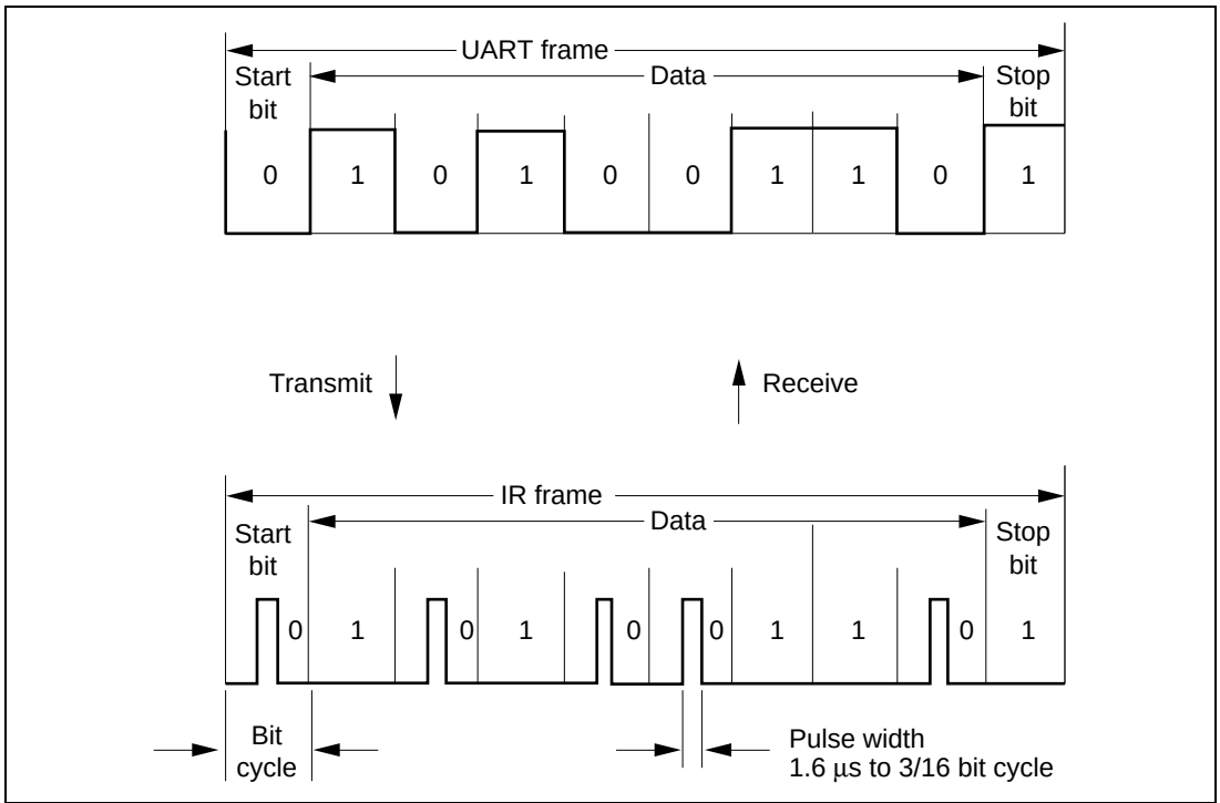
Figure 15.34 IrDA Transmit/Receive Operations
