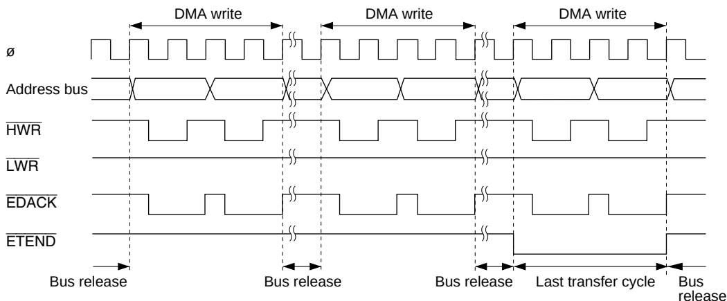
Figure 8.25 Example of Single Address Mode (Word Write) Transfer
