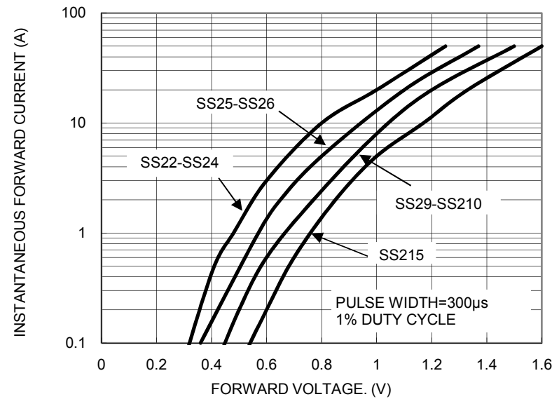
FIG. 3 TYPICAL FORWARD CHARACTERISTICS
