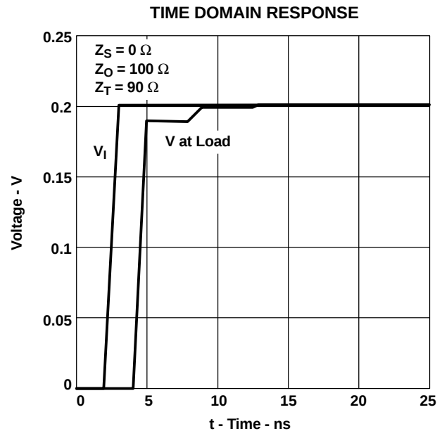
Figure 15. High-Source Impedance
