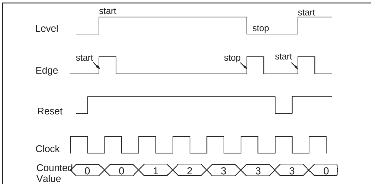
Figure 7.1. Timer Functionalities
