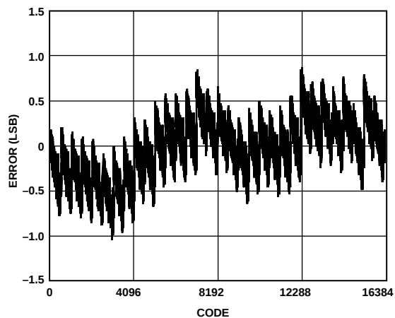
Figure 15. Typical INL
