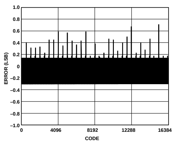
Figure 16. Typical DNL
