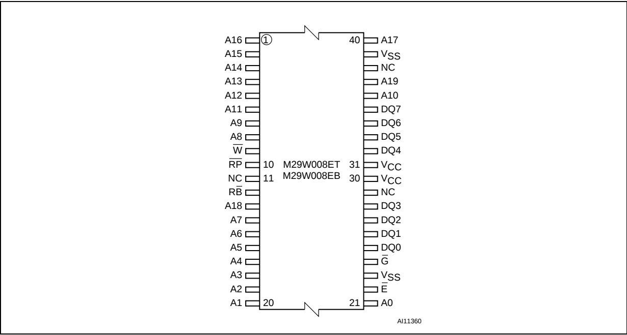
Figure 3. TSOP Connections
