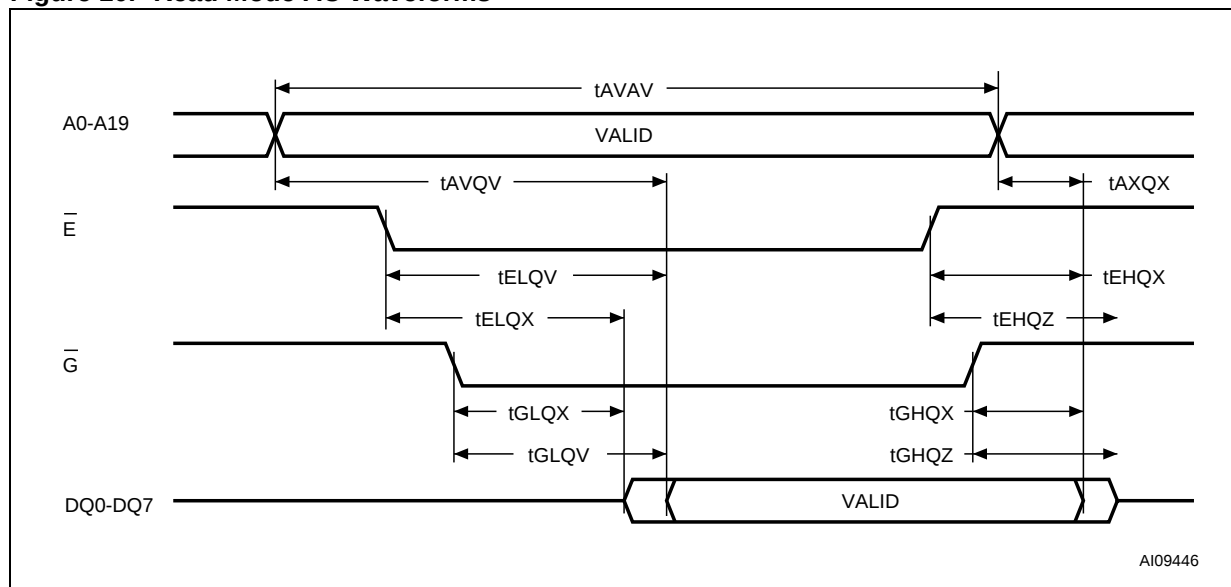
Figure 10. Read Mode AC Waveforms
