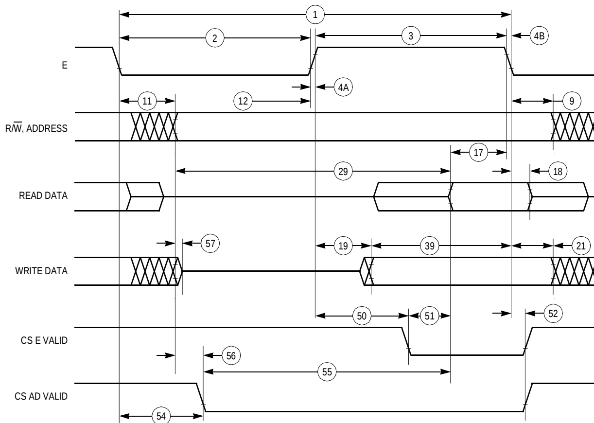
Figure 12-9. Expansion Bus Timing
