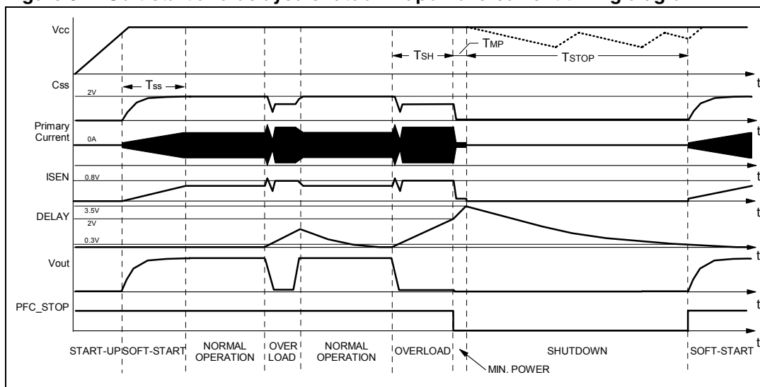
Figure 32. Soft-start and delayed shutdown upon overcurrent timing diagram
