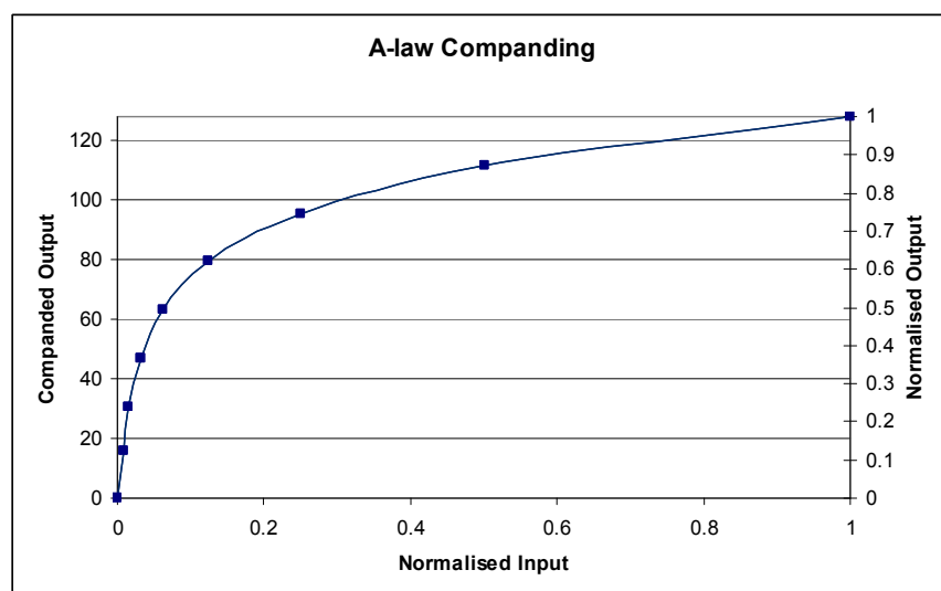
Figure 51 A-Law Companding
