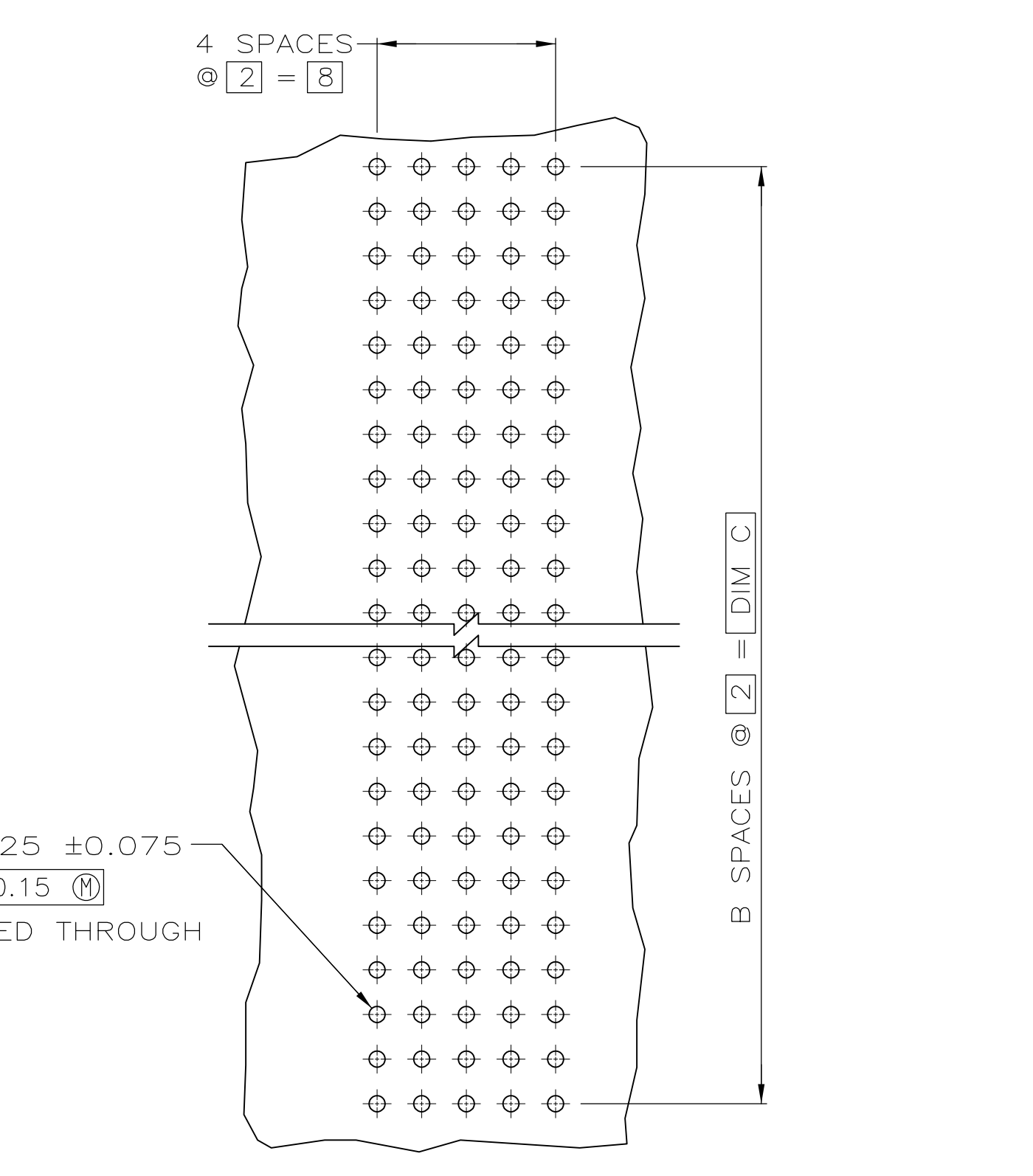
RECOMMENDED CIRCUIT PATTERN (COMPONENT SIDE)
