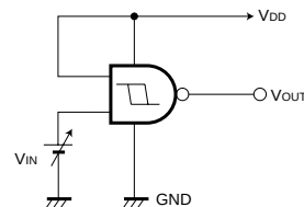
Fig. 3 Hysteresis voltage
