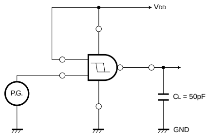
Fig. 2 Switching characteristic
