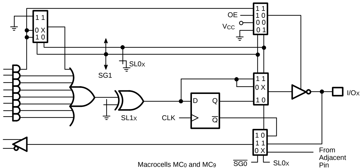
PALCE24V10 Macrocell
