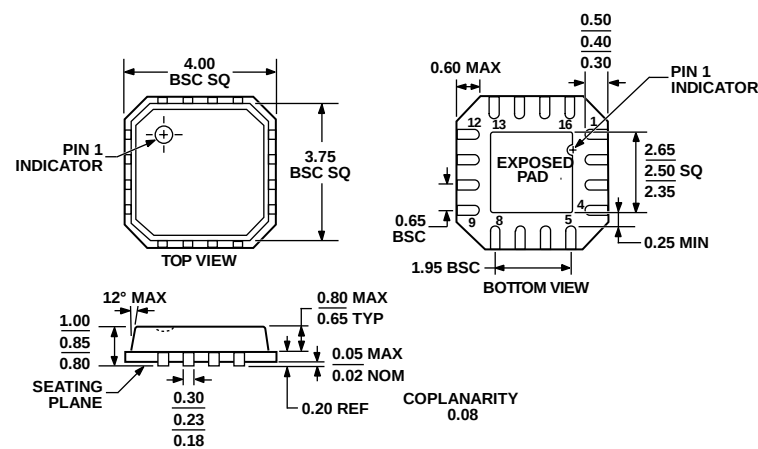
COMPLIANT TO JEDEC STANDARDS MO-220-VGFC. Figure 47. 16-Lead Frame Chip Scale Package [LFCSP_VQ] 4 mm x 4 mm Very Thin Quad (CP-16-13) Dimensions shown in millimeters
