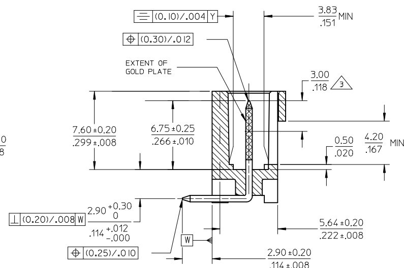
SECTION K-K
