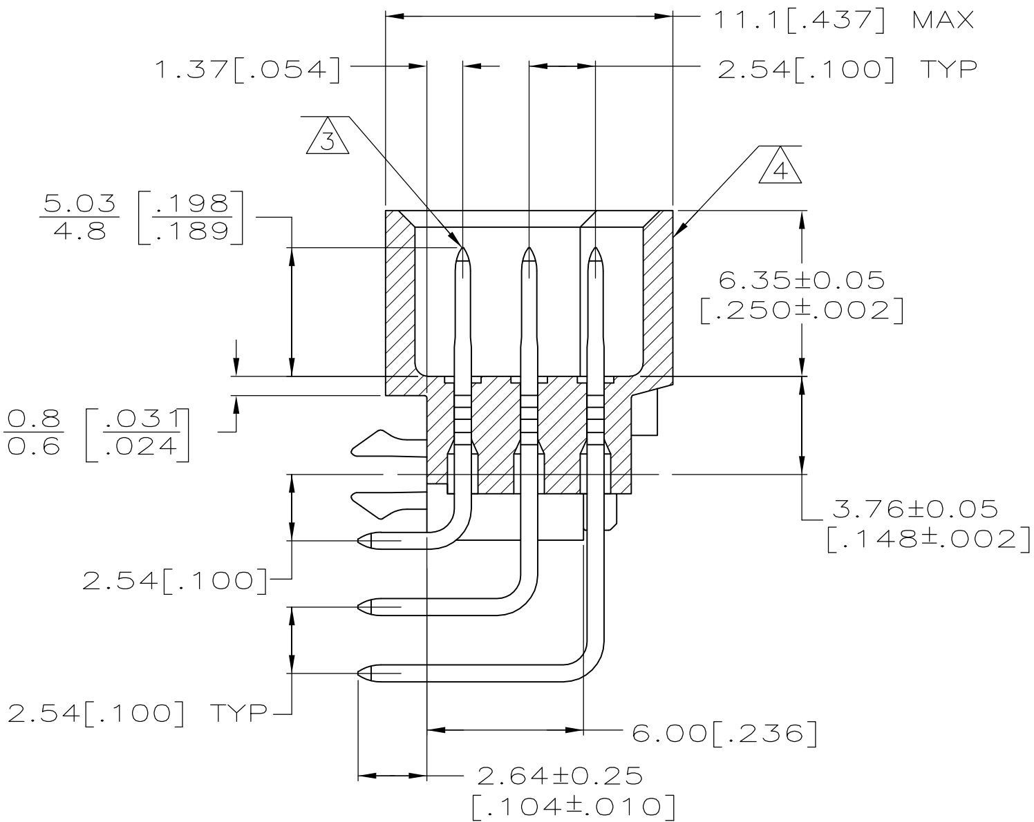
SECTION X-X
