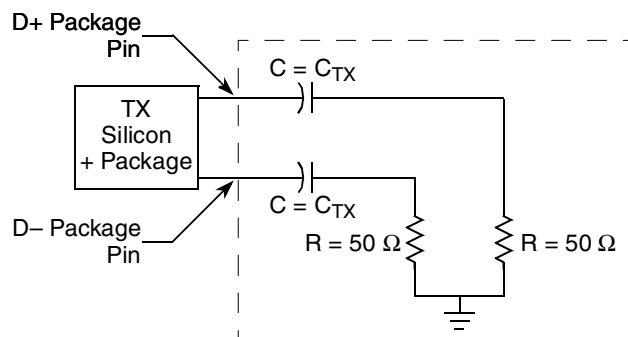
Figure 57. Compliance Test/Measurement Load
