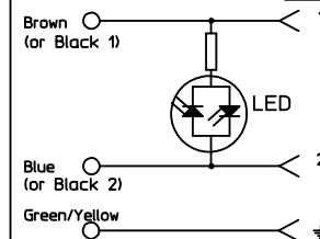
ELECTRICAL DIAGRAM [A1]
