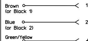
ELECTRICAL DIAGRAM [00] WITHOUT LED
