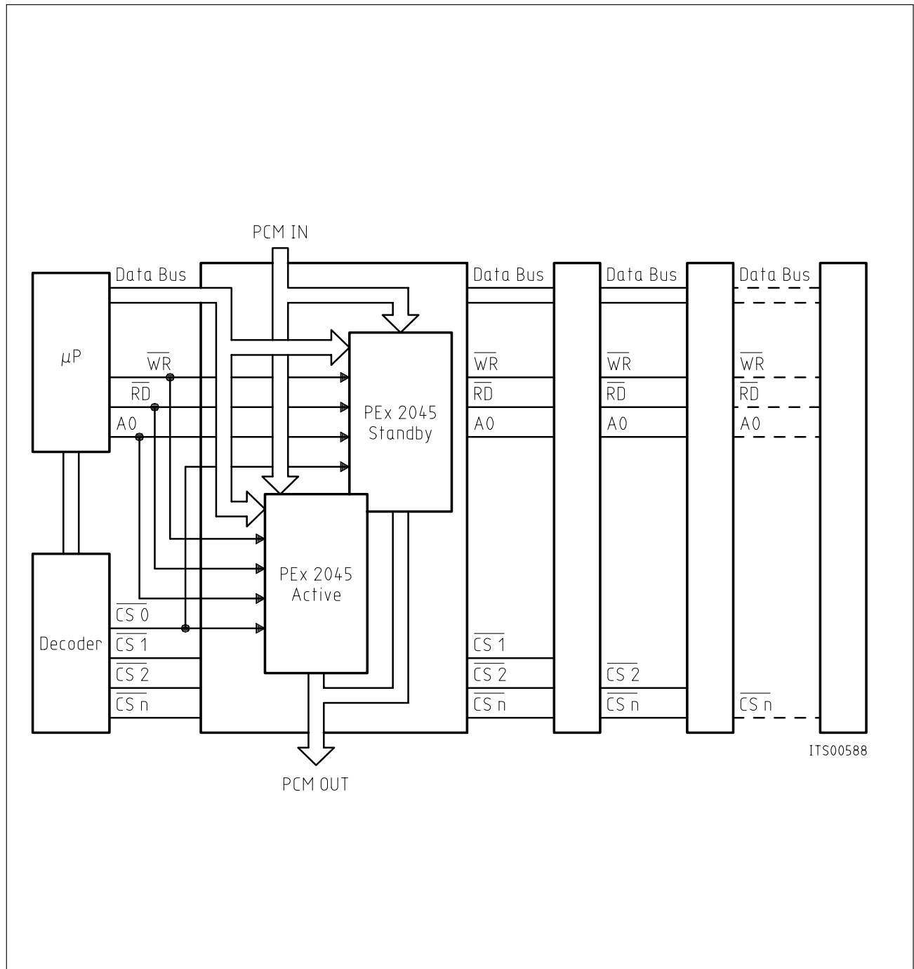
Figure 20 Device Setup in Redundant Systems
