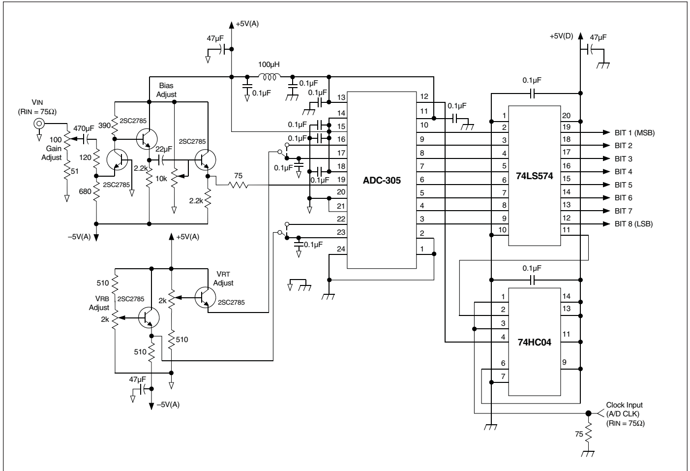
Figure 5. Typical Connection Diagram
