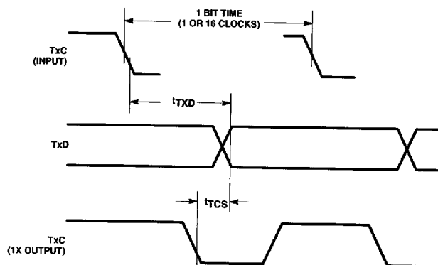
Figure 6. Transmitter External Clocks
