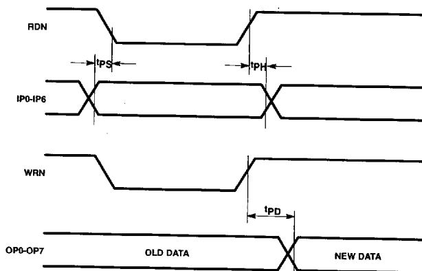
Figure 3. Port Timing
