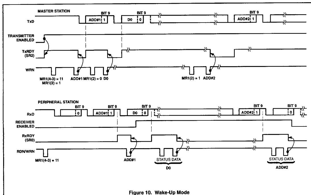
Figure 10. Wake-Up Mode
