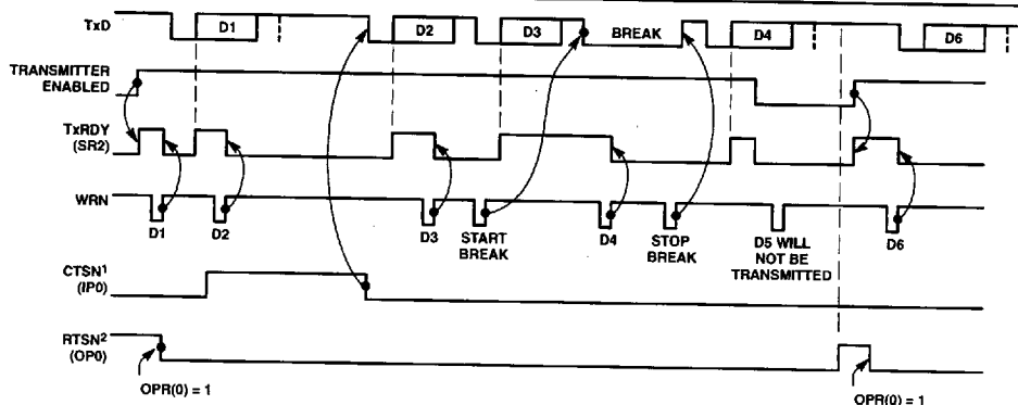
Figure 8. Transmitter Timing
