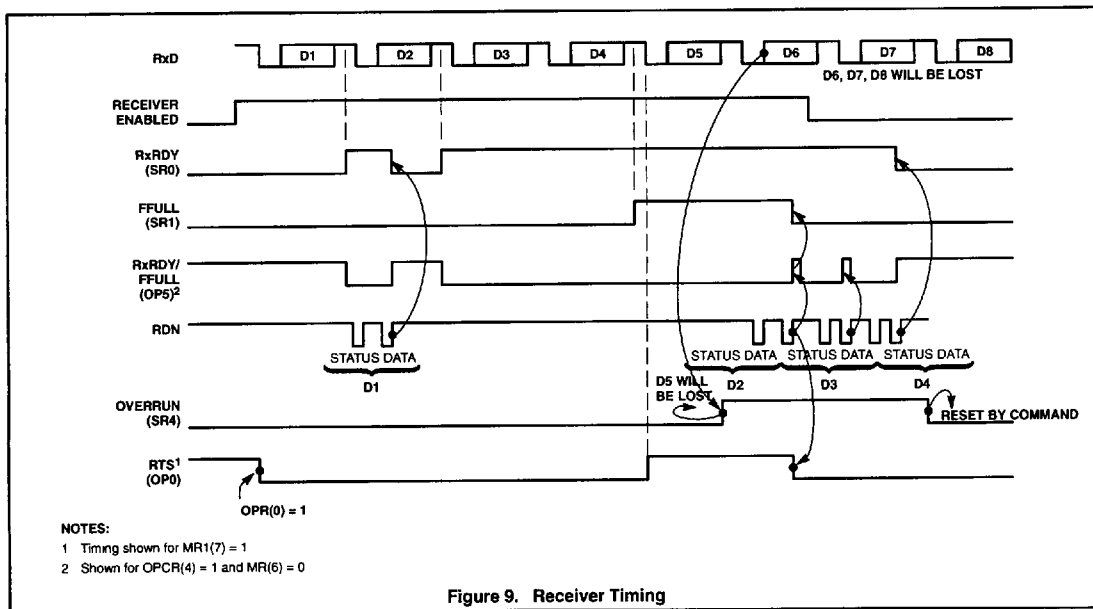
Figure 9. Receiver Timing
