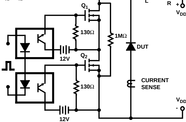
FIGURE 7. AVALANCHE ENERGY TEST CIRCUIT
