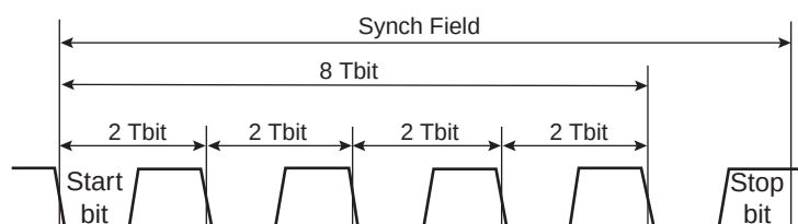
Figure 25-29. Sync Field
