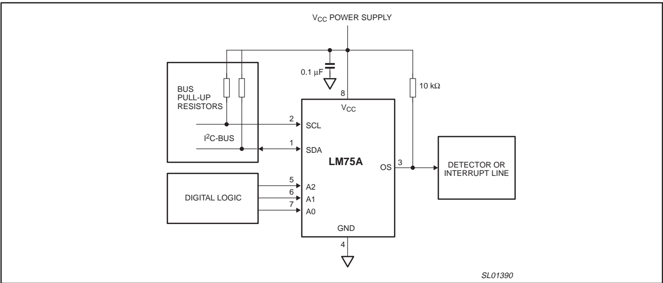
Figure 3. Typical connection.
