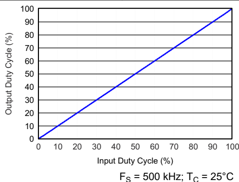
Figure 6-5. Output Duty Cycle vs Input Duty Cycle
