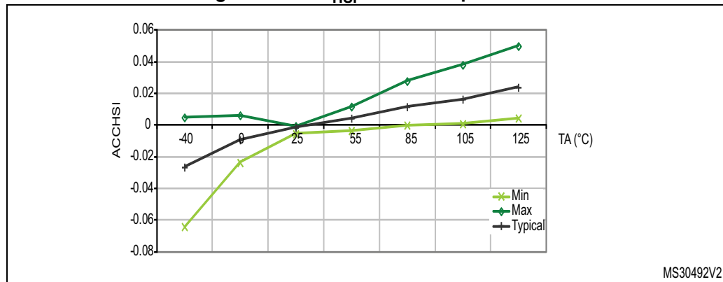
Figure 31. ACC_{HSI} versus temperature
