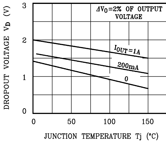
V_D - T_j
