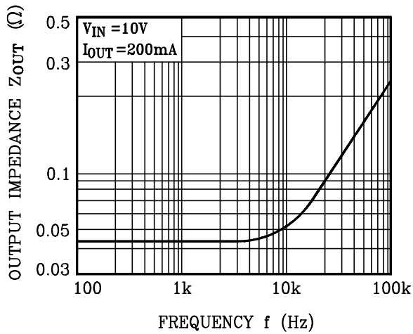
Z_{OUT} - f
